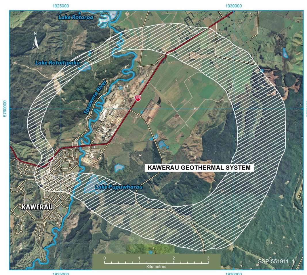
Figure 1 The location of the Kawerau Geothermal System (Based on inferred resistivity boundary) (Based on Milichich et al 2015, after Allis 1997).
