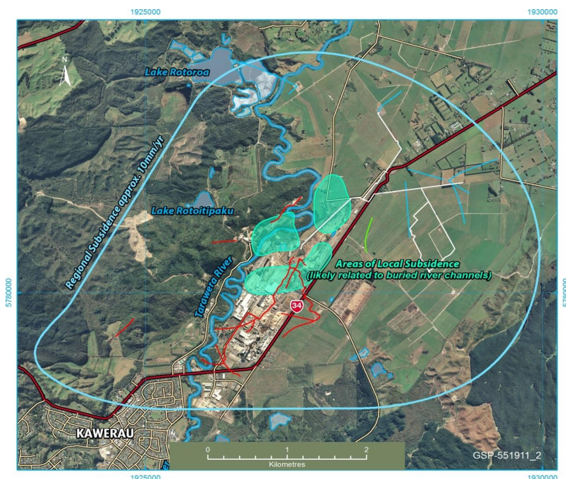
Figure 3.3 General patterns of subsidence in the Kawerau area.
